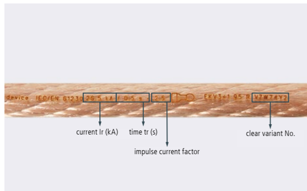
Required markings on the EaS device (see laser engraving)
