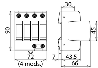
Dimension drawing DG M TT 275 NL
