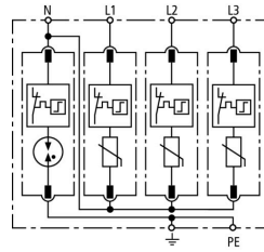
Basic circuit diagram DG M TT 275 NL
