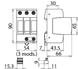
Dimension drawing DG M TNC CI 275 FM
