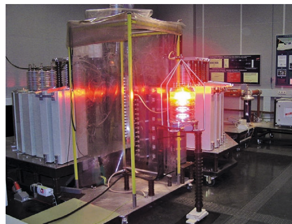
Figure 13 Customer-specific testing in the impulse current laboratory
